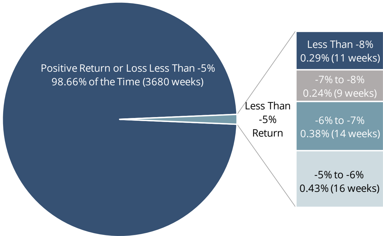
S&P 500 Weekly Returns
