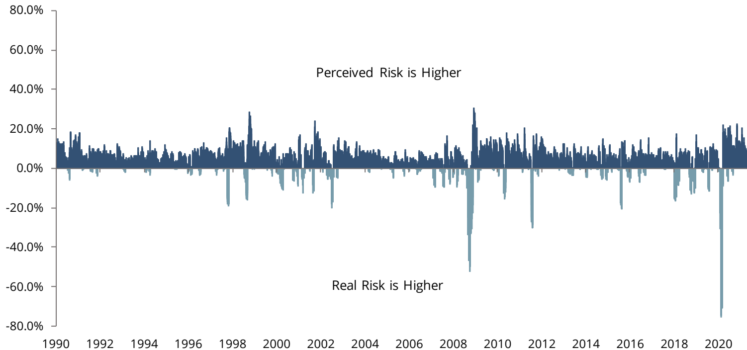
Difference between VIX and realized Vol 20 (trading) days later (1/1/1990 - 6/30/2021)
